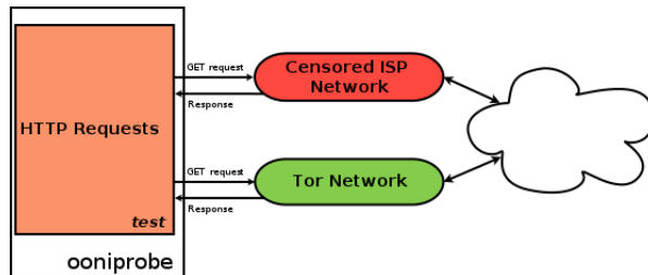
Figure 1: Ooniprobe HTTP request test diagram
